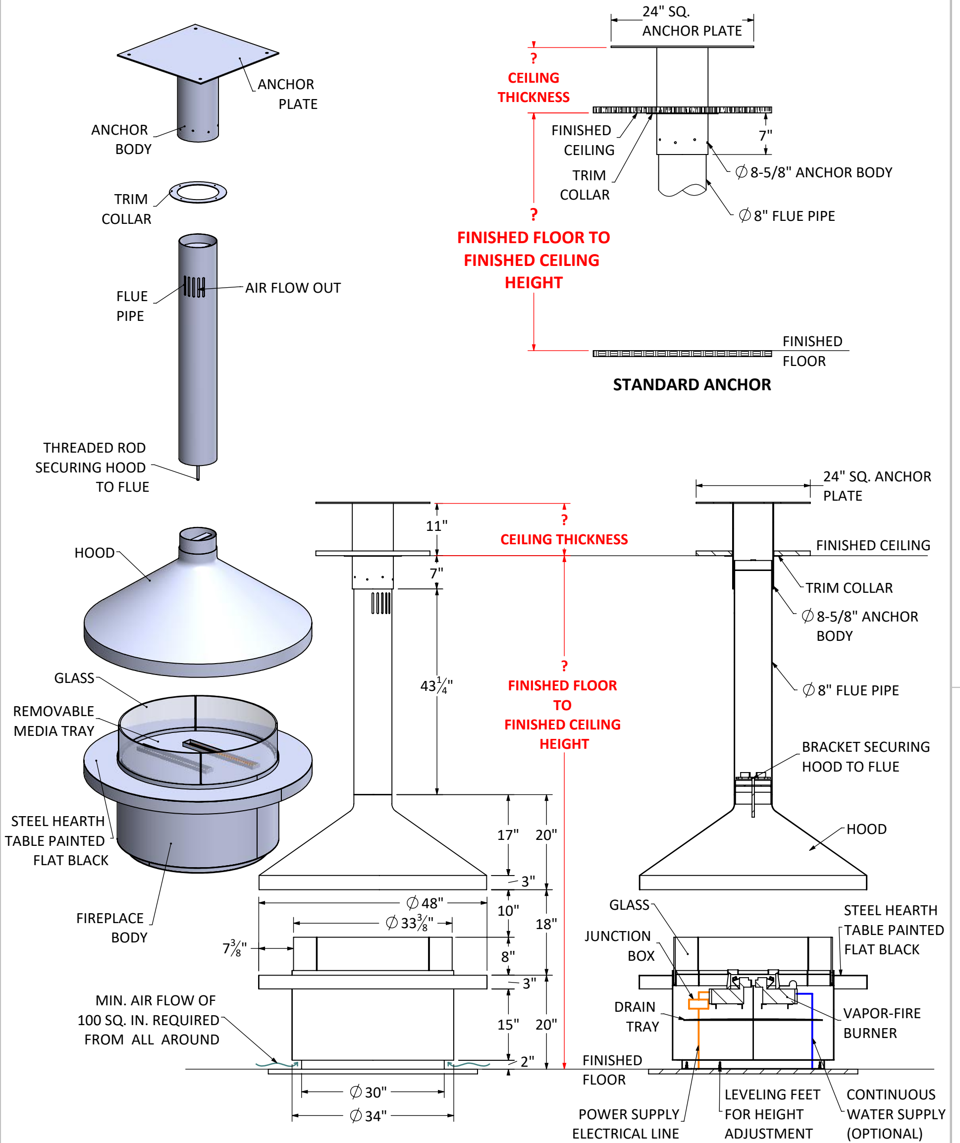
SECTION VIEW SCALE 1:20
