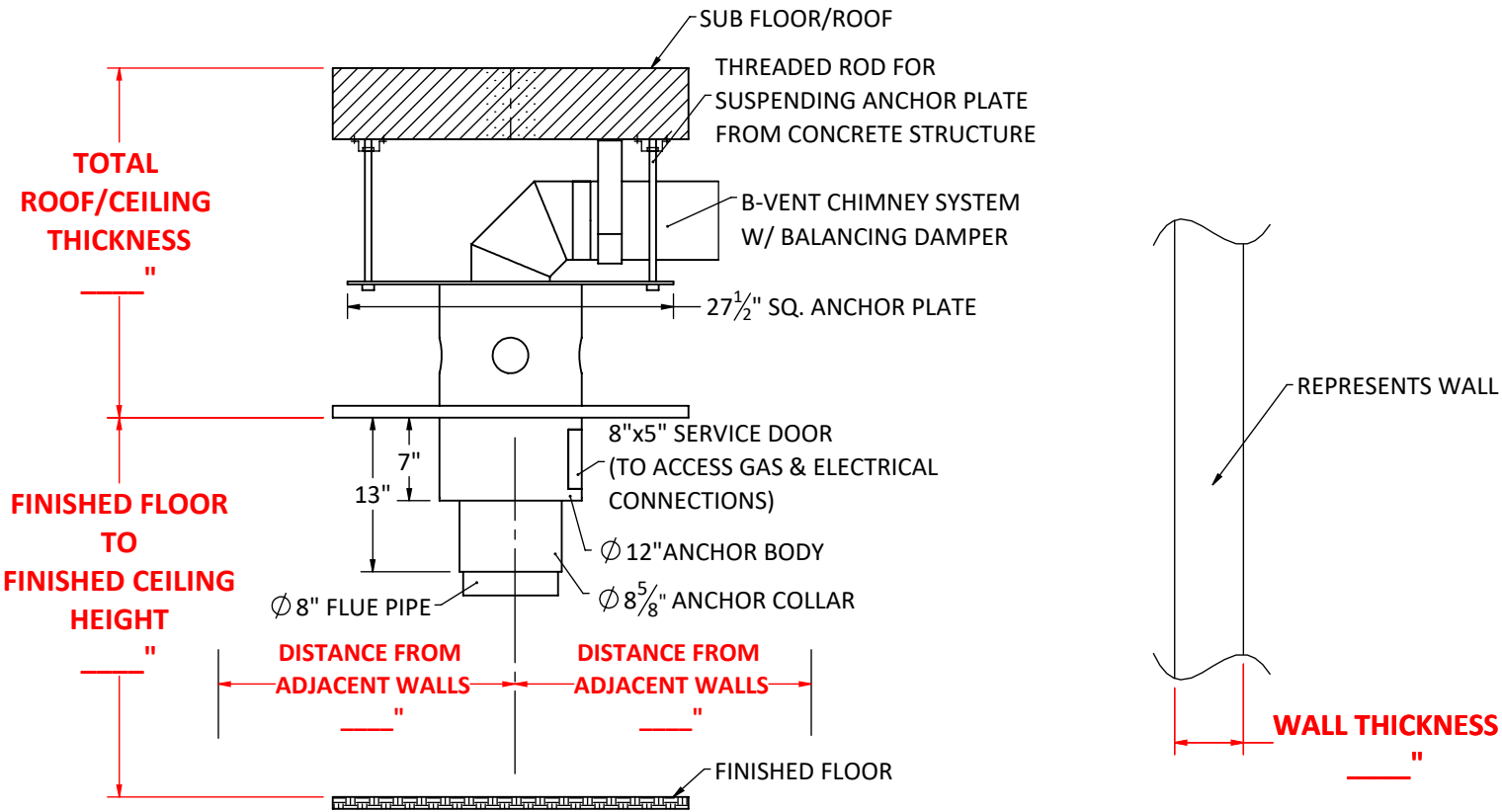
OPTION B - SUSPENDED FROM CONCRETE
