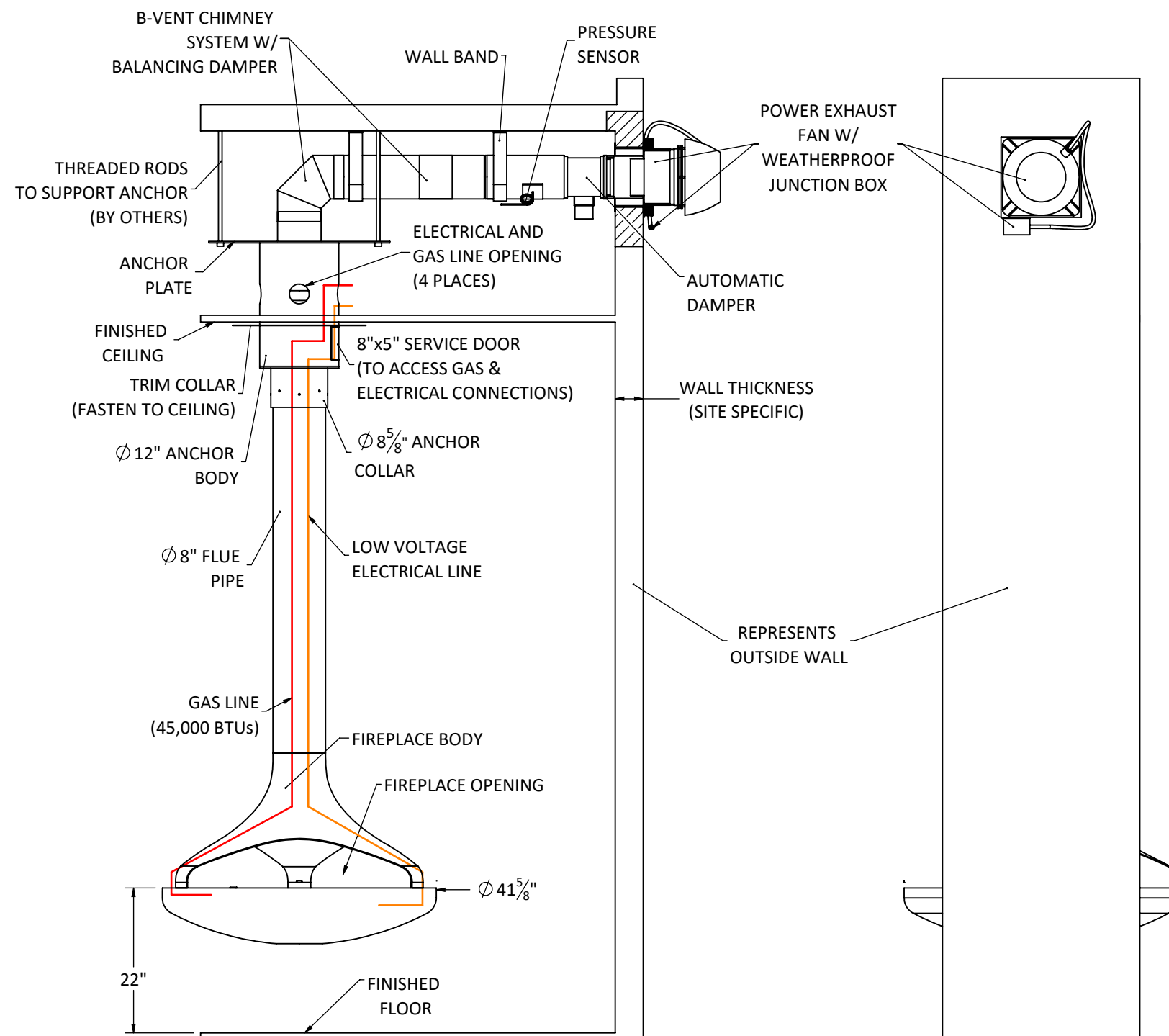
FRONT ELEVATION
