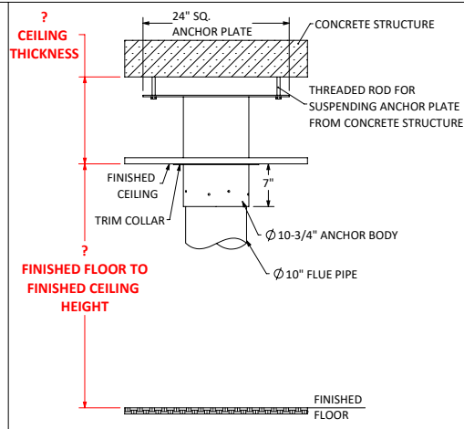
OPTION B - SUSPENDED FROM CONCRETE
