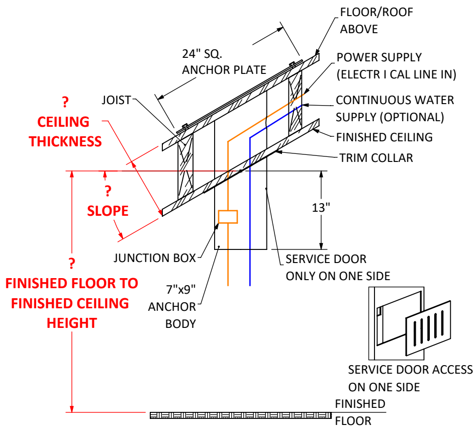
OPTION A - SLOPED DROP FROM ABOVE
