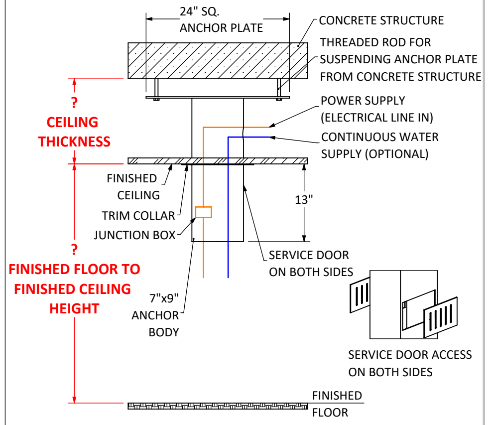
OPTION B - SUSPENDED FROM CONCRETE
