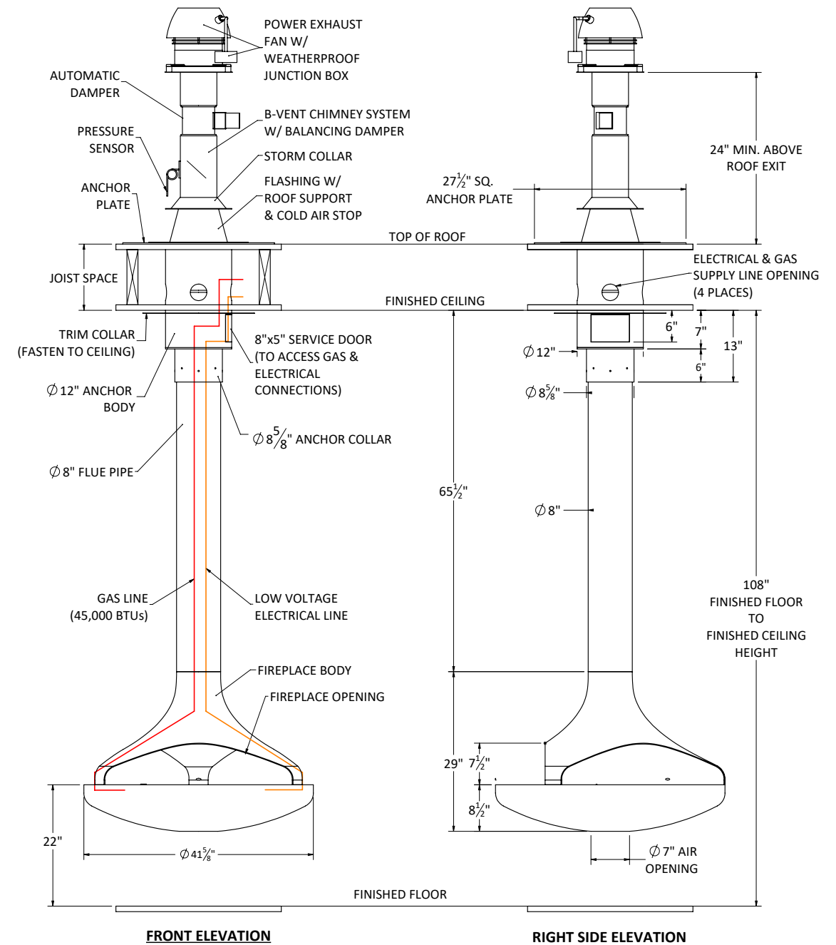
FRONT ELEVATION RIGHT SIDE ELEVATION Shown with standard 9 ft. ceiling application and flat anchor option.
