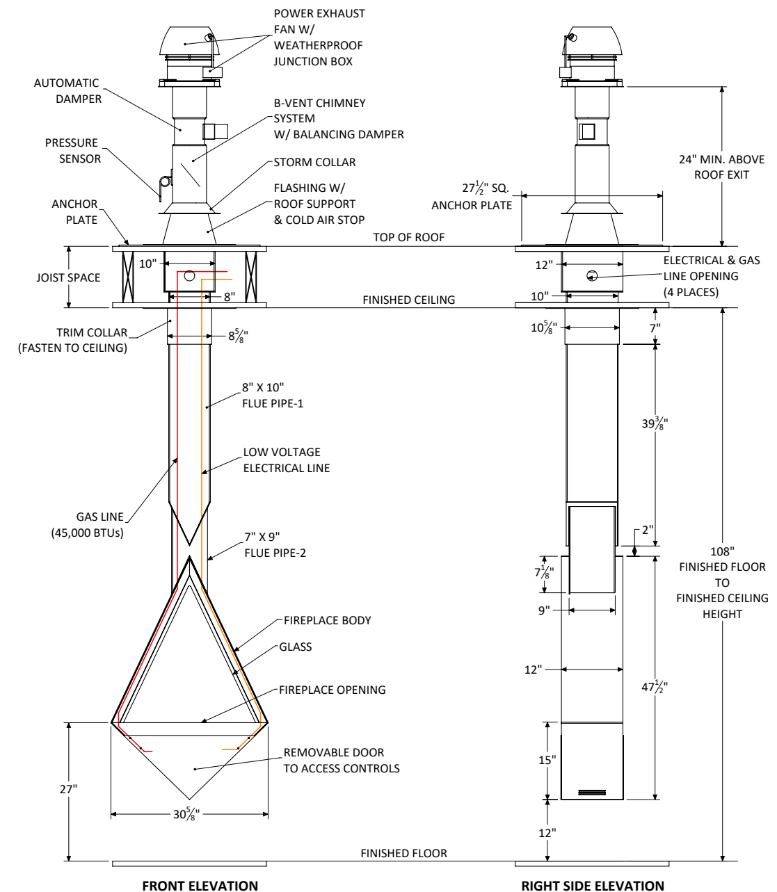
Shown with standard 9 ft. ceiling application and flat anchor option.
