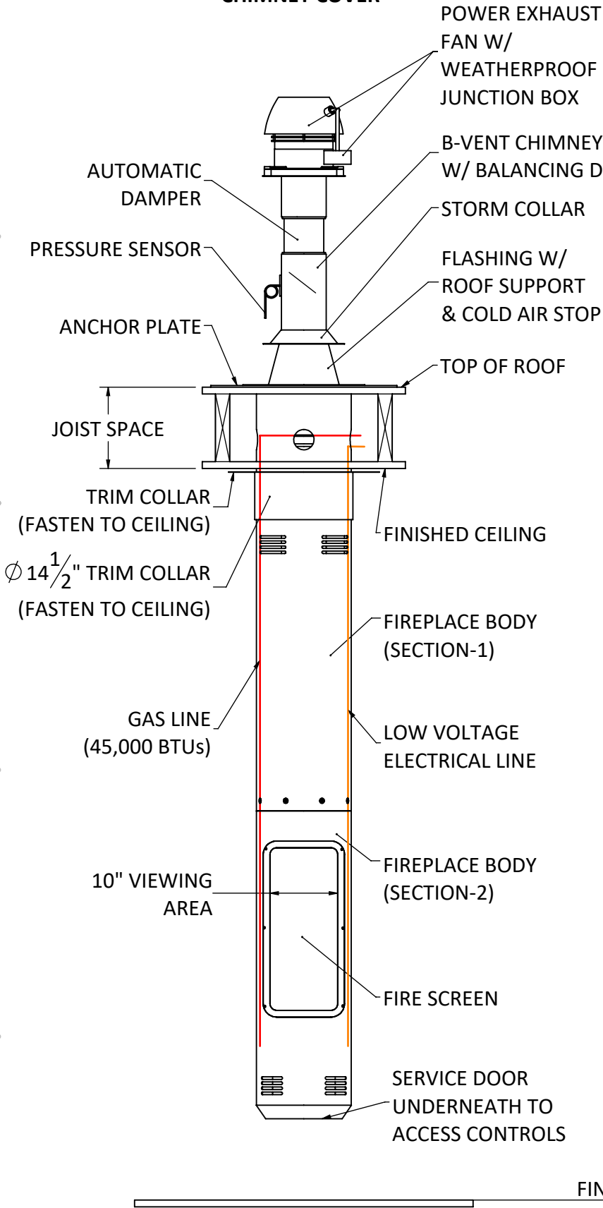
FRONT ELEVATION
