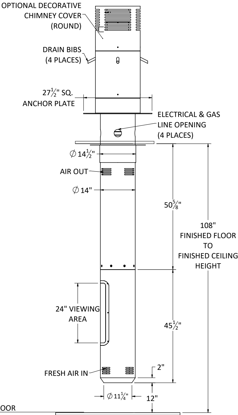
SIDE ELEVATION
