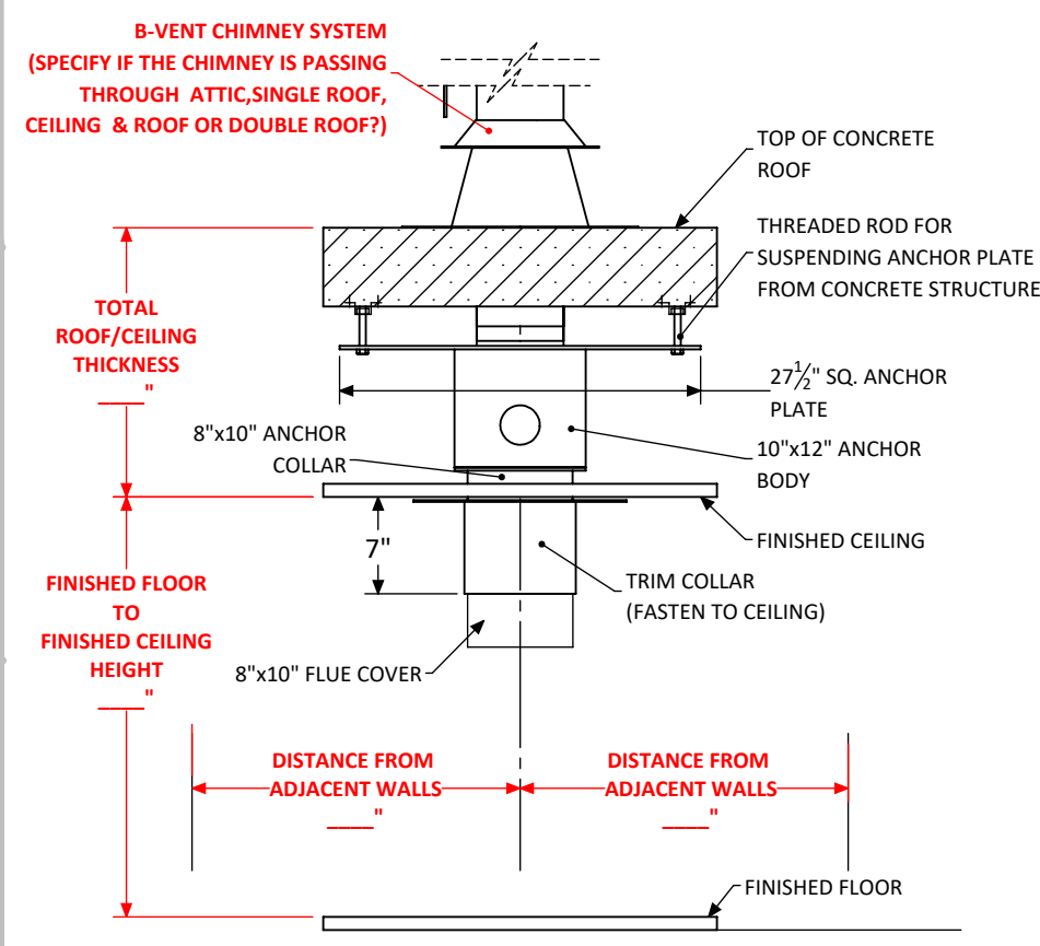
OPTION C - SUSPENDED FROM CONCRETE
