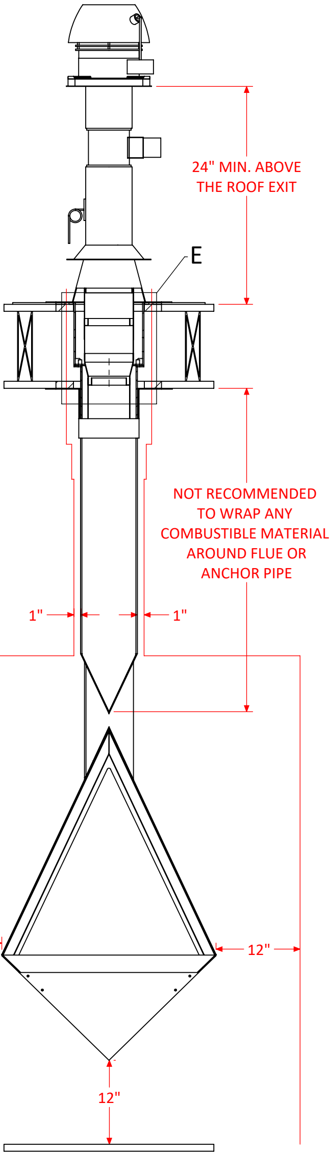
FRONT ELEVATION
