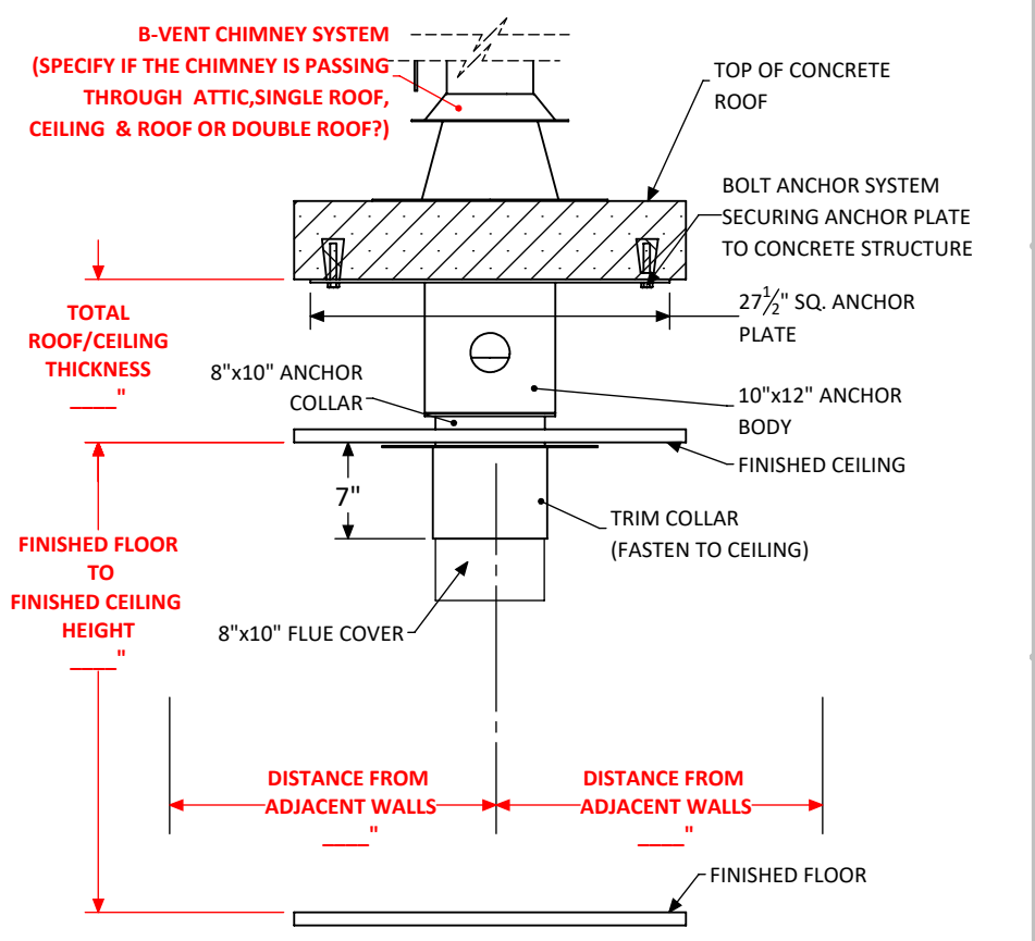
OPTION D - ATTACHED BELOW CONCRETE
