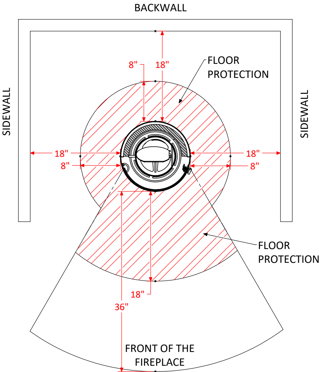
CLEARANCE TO COMBUSTIBLES AROUND FIREPLACE BODY & FLOOR PROTECTION REQUIREMENTS
