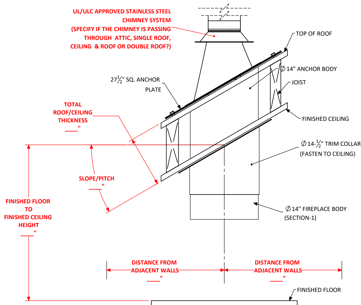
OPTION B - SLOPED DROP FROM ABOVE
