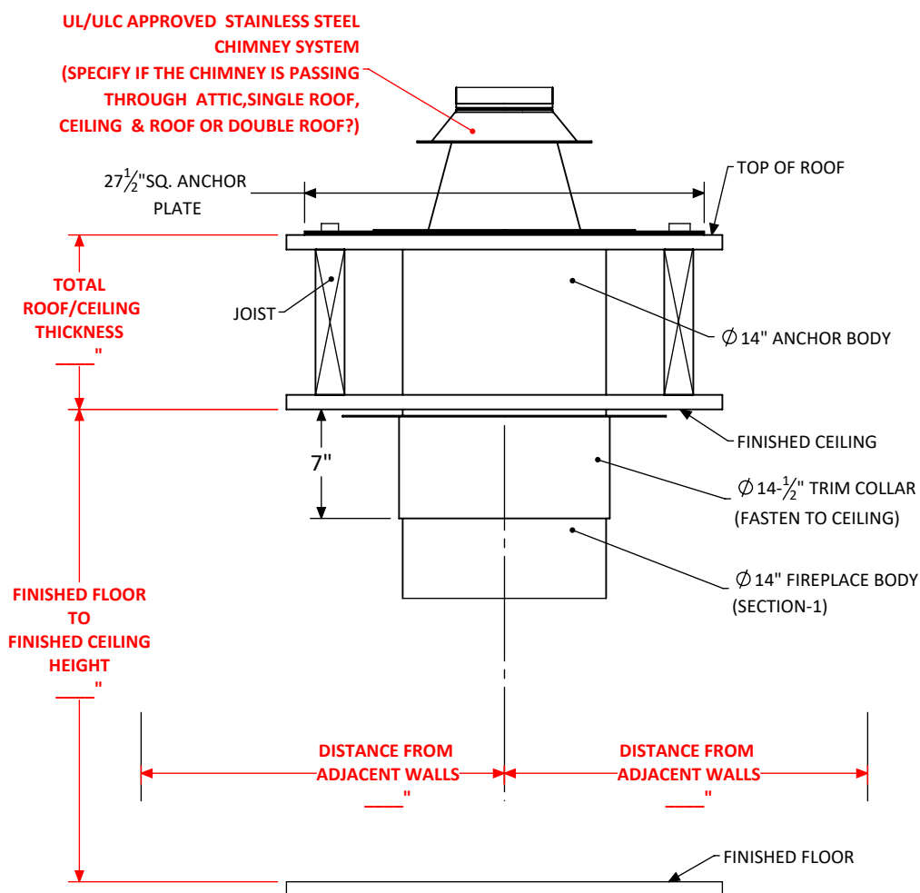
OPTION A - FLAT ROOF DROP FROM ABOVE
