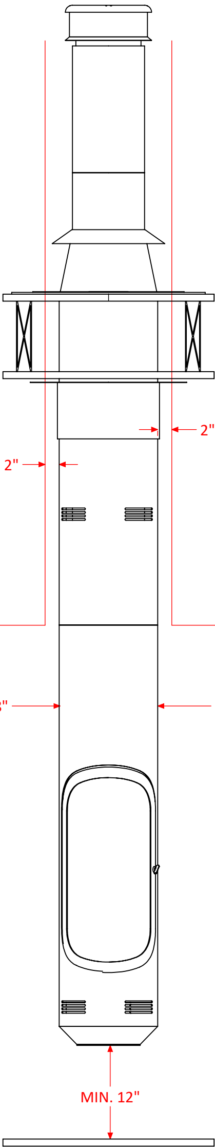
FRONT ELEVATION
