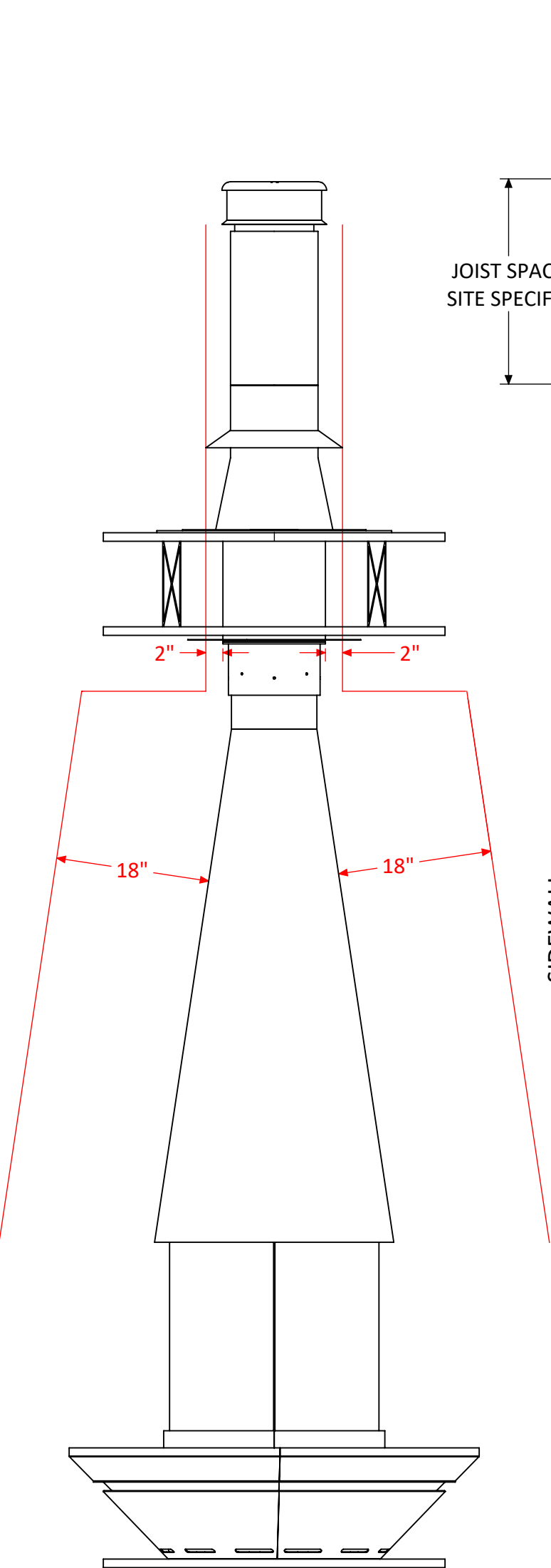
FRONT ELEVATION
