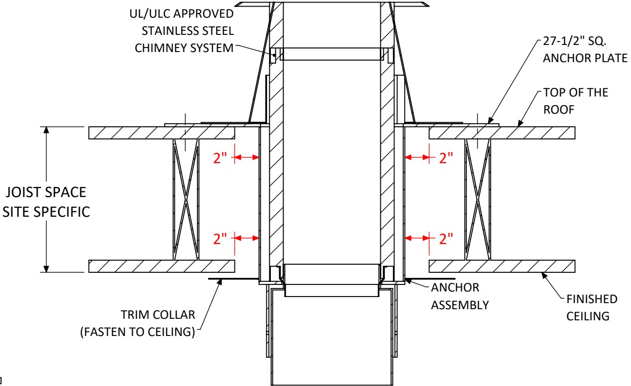
CLEARANCE TO COMBUSTIBLES AT CEILING AND ROOF
