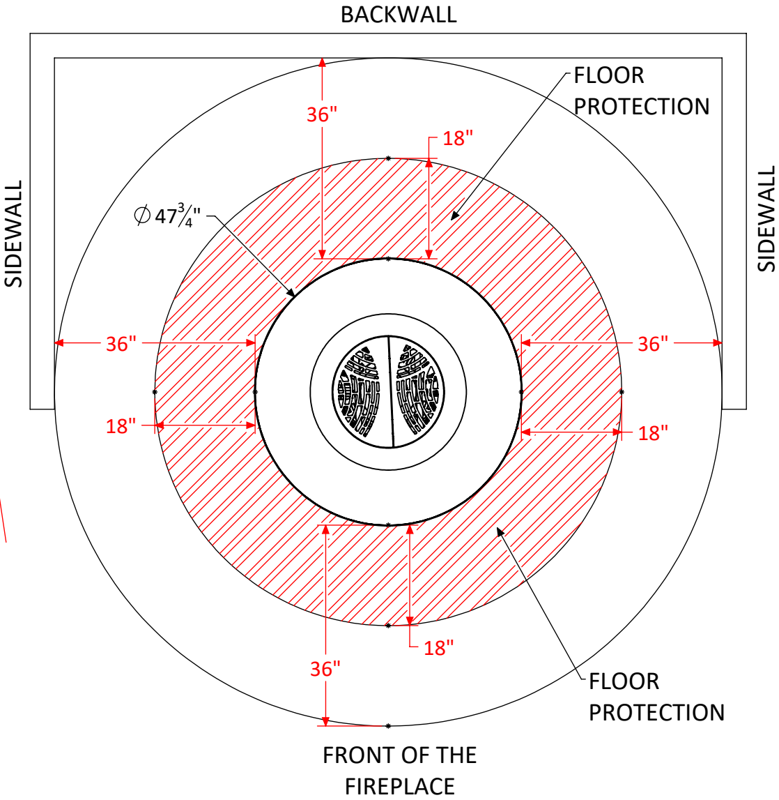
TOP VIEW
