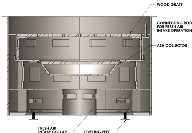
TYPICAL FLOOR MODEL SECTION VIEW SAMPLE IMAGE ONLY
