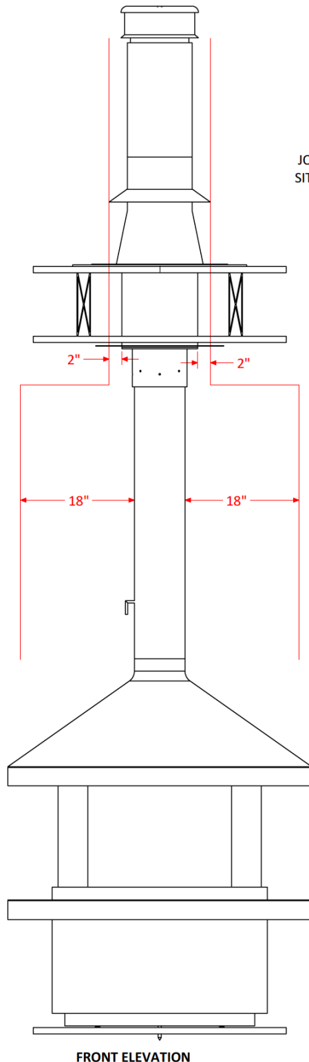
FRONT ELEVATION
