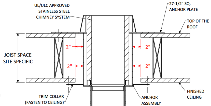
CLEARANCE TO COMBUSTIBLES AT CEILING AND ROOF
