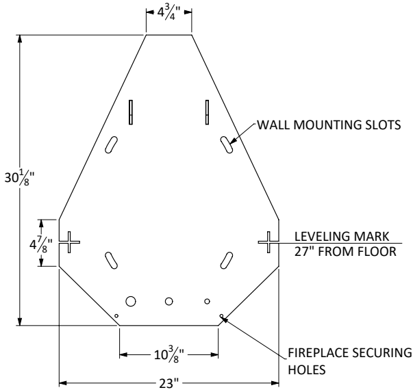
Standard Wall Mounting Plate shown.
