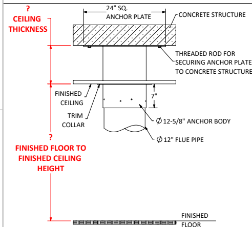
OPTION C - ATTACHED BELOW CONCRETE
