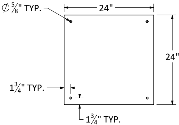
ANCHOR PLATE 24" SQ. x 0.25" THK.
