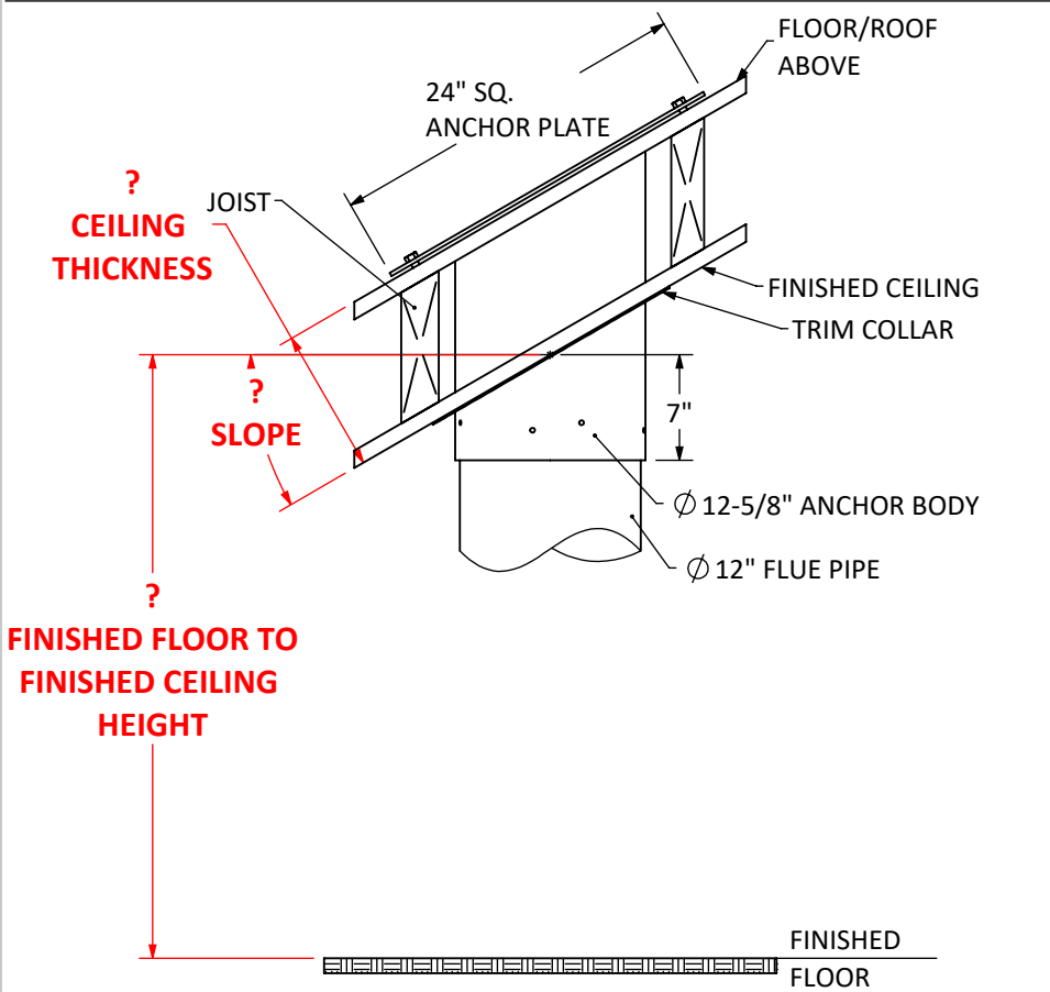
OPTION A - SLOPED DROP FROM ABOVE
