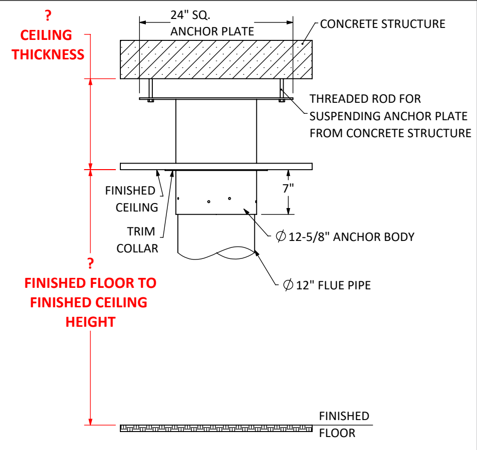
OPTION B - SUSPENDED FROM CONCRETE
