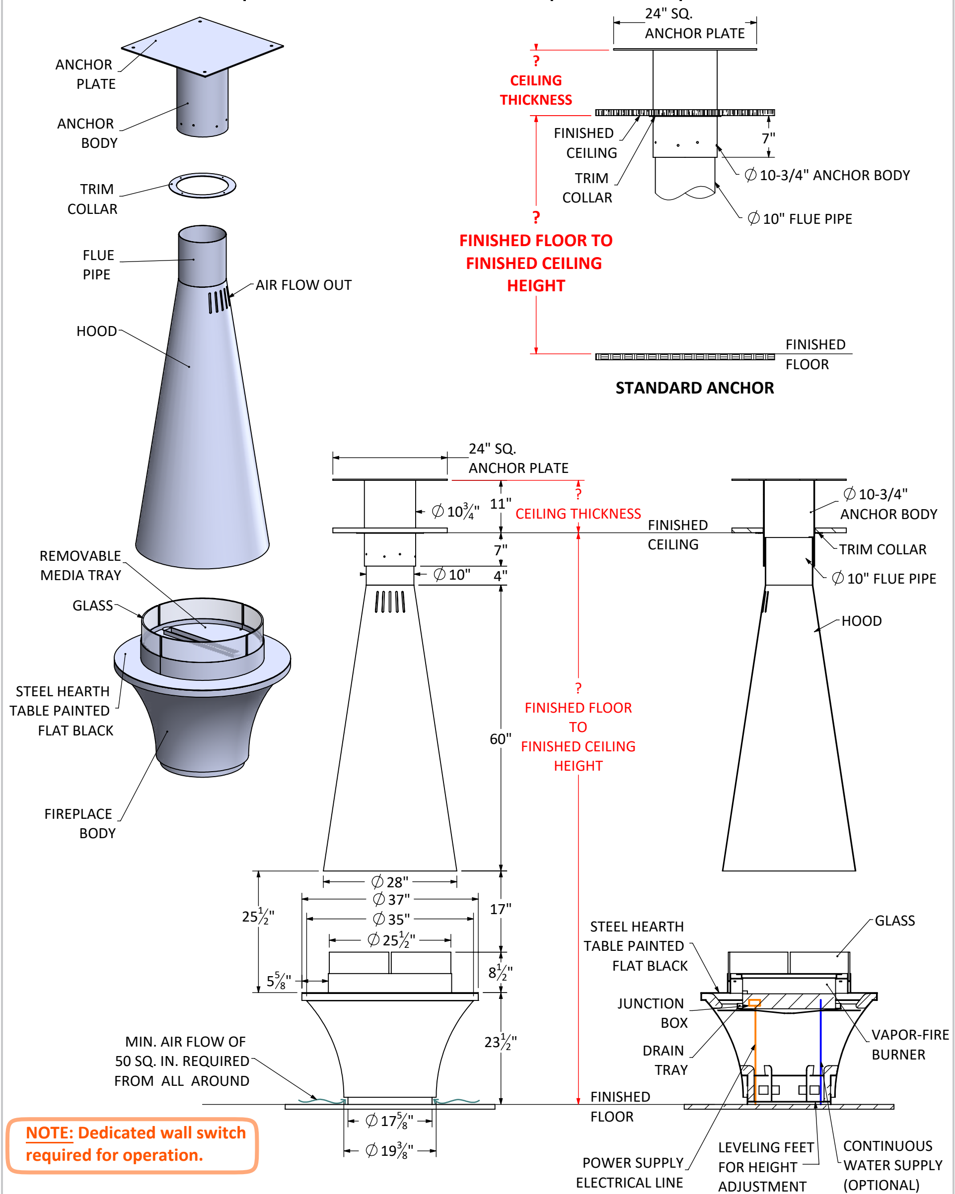
SECTION VIEW SCALE 1:20
