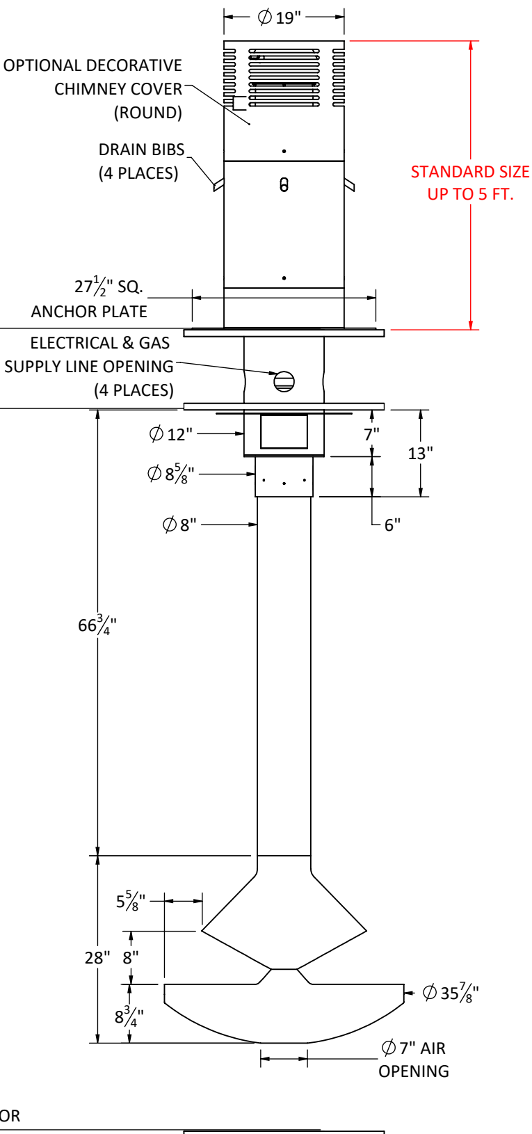
SIDE ELEVATION
