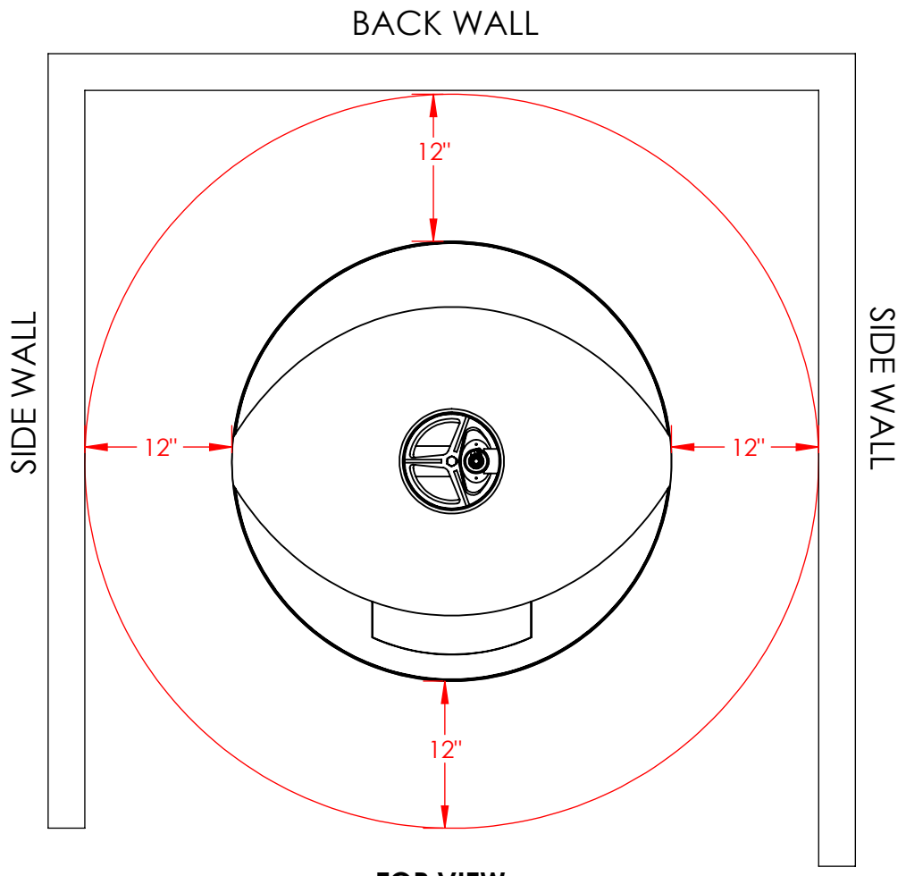
TOP VIEW CLEARANCE TO COMBUSTIBLES AROUND FIREPLACE BODY
