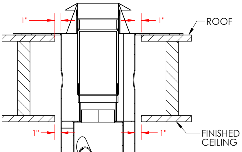
CLEARANCE TO COMBUSTIBLES AT CEILING AND ROOF
