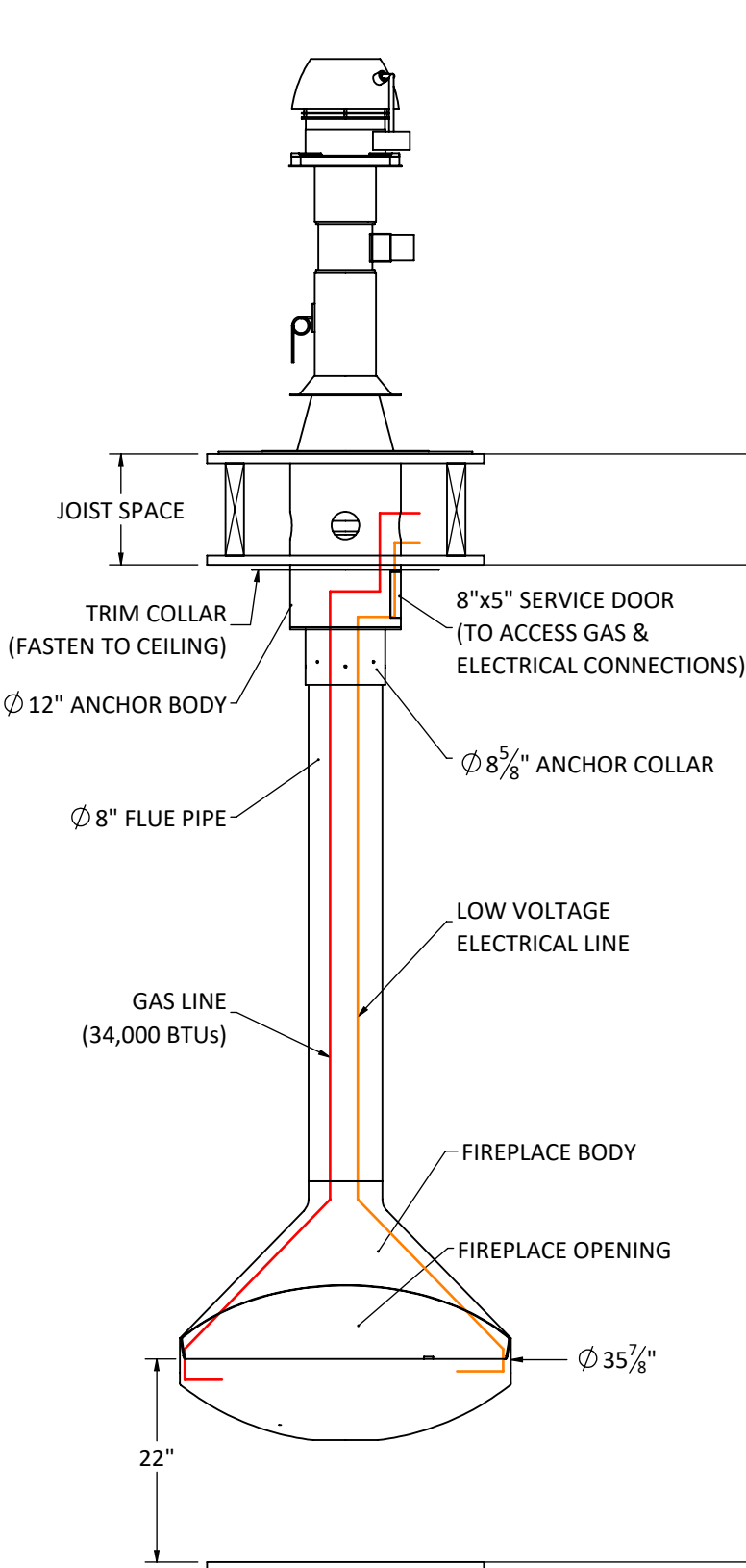
FRONT ELEVATION
