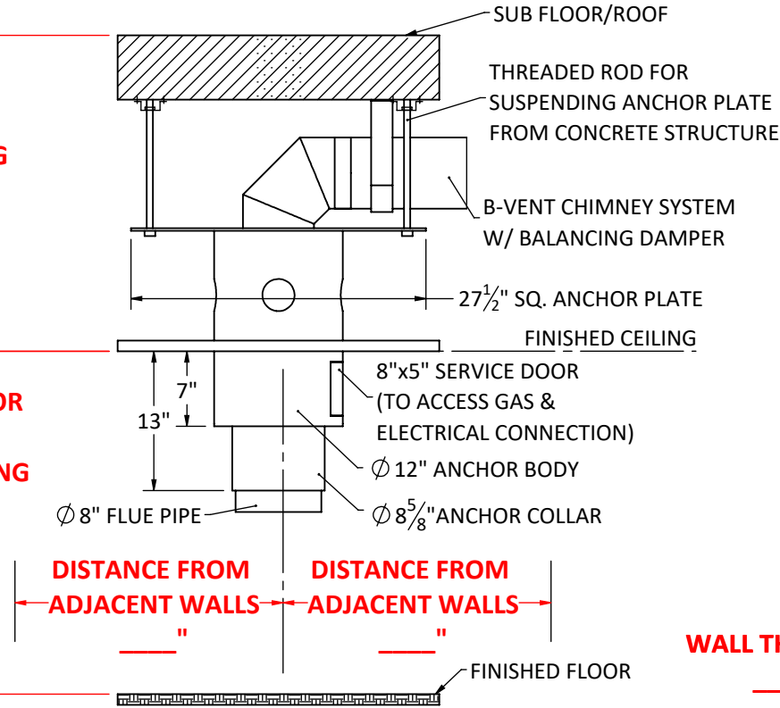
OPTION B - SUSPENDED FROM CONCRETE
