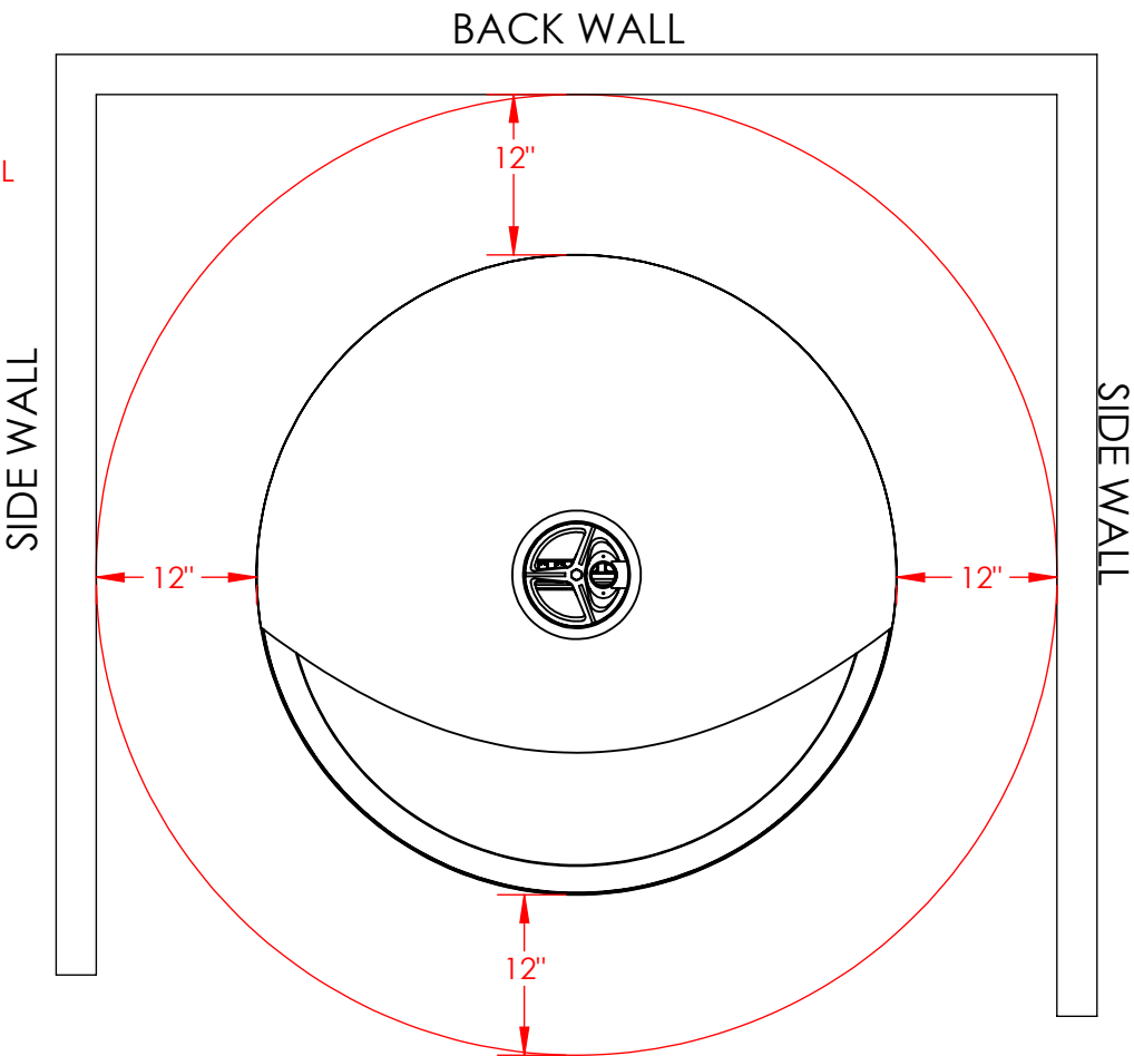
CLEARANCE TO COMBUSTIBLES AROUND FIREPLACE BODY
