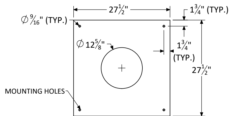
STANDARD ANCHOR PLATE- 1/4" THICK.
