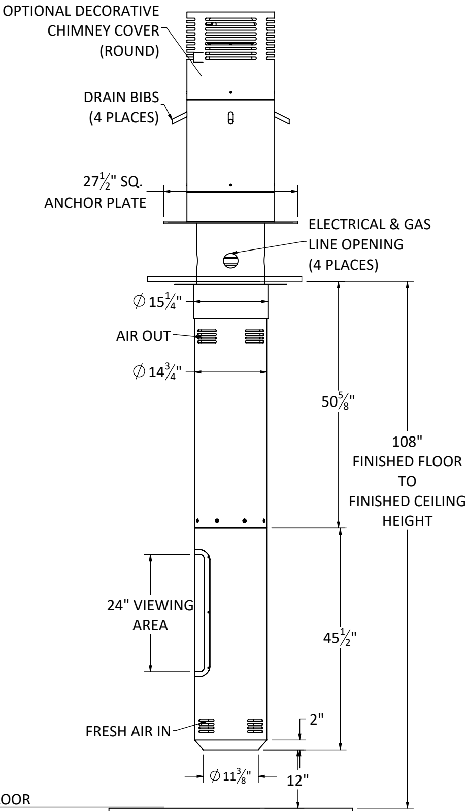
SIDE ELEVATION
