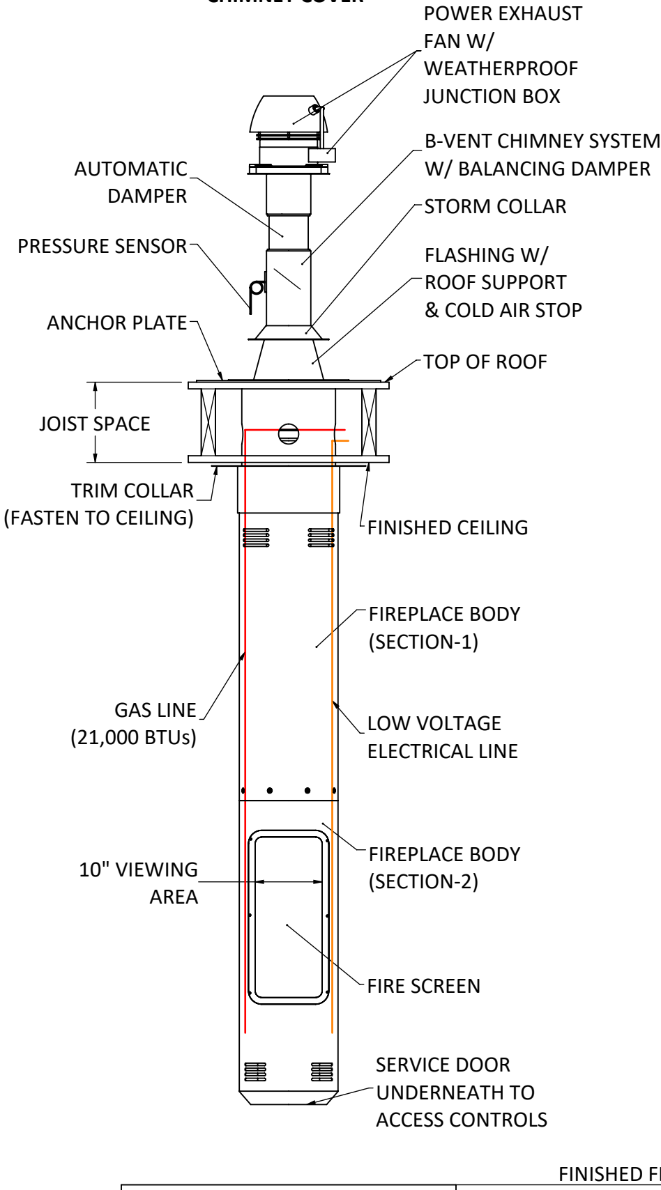
FRONT ELEVATION
