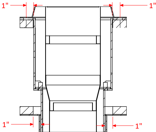
CLEARANCE TO COMBUSTIBLES AT CEILING AND ROOF
