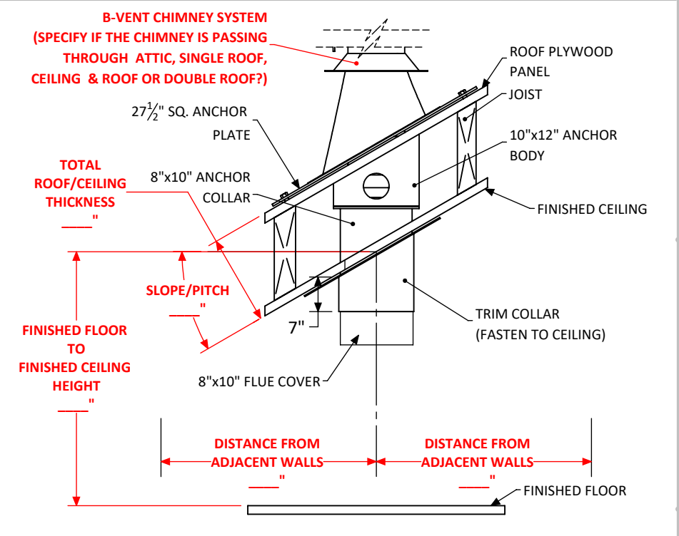
OPTION B - SLOPED DROP FROM ABOVE
