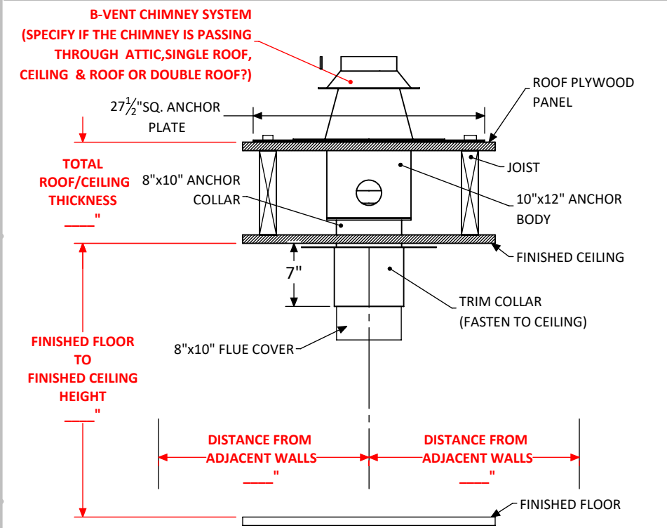
OPTION A - FLAT ROOF DROP FROM ABOVE
