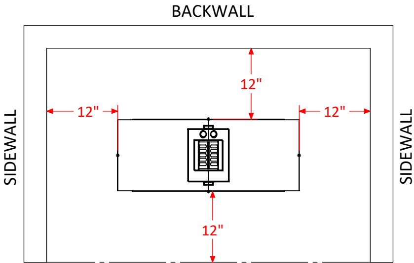
CLEARANCE TO COMBUSTIBLES AROUND FIREPLACE BODY
