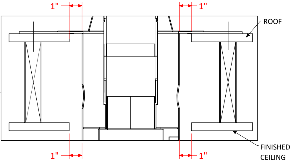
CLEARANCE TO COMBUSTIBLES AT CEILING AND ROOF
