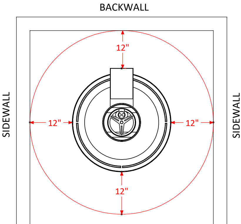
FRONT OF THE FIREPLACE TOP VIEW
