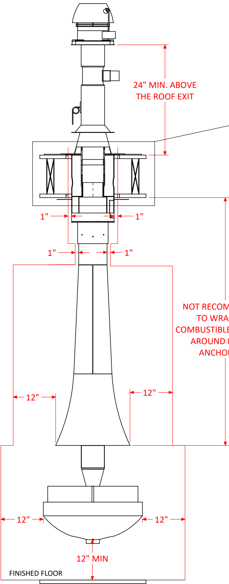
FRONT ELEVATION
