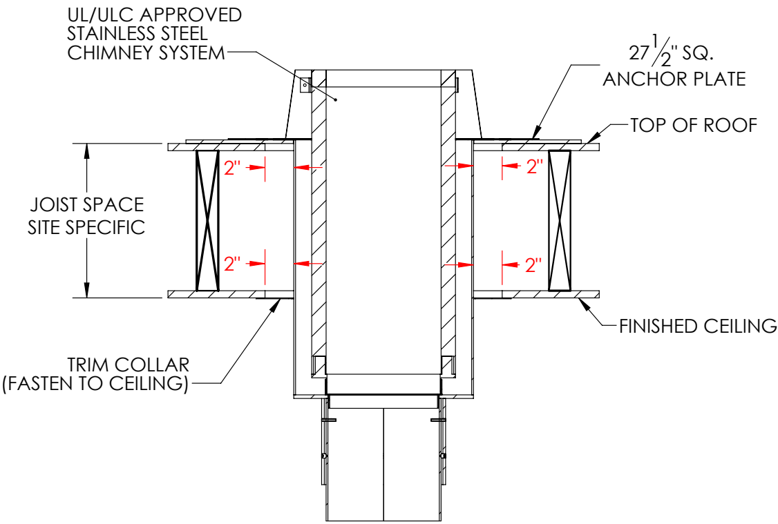
CLEARANCE TO COMBUSTIBLES AT CEILING AND ROOF
