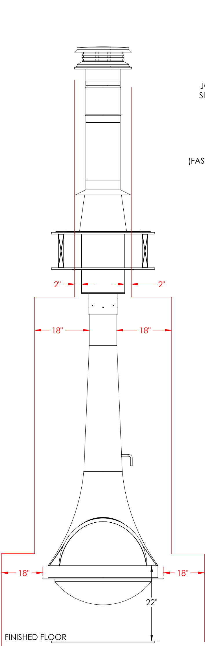
FRONT ELEVATION
