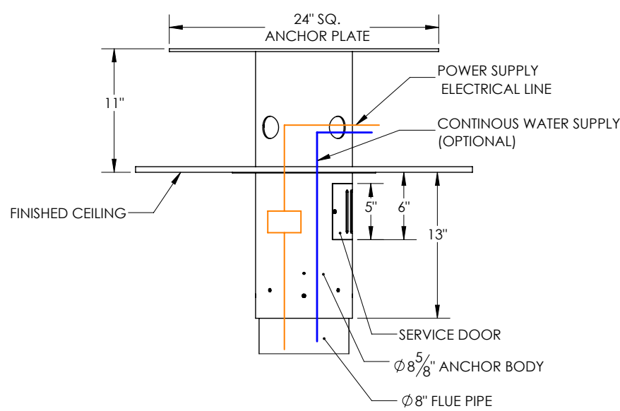
STANDARD FLAT ANCHOR
