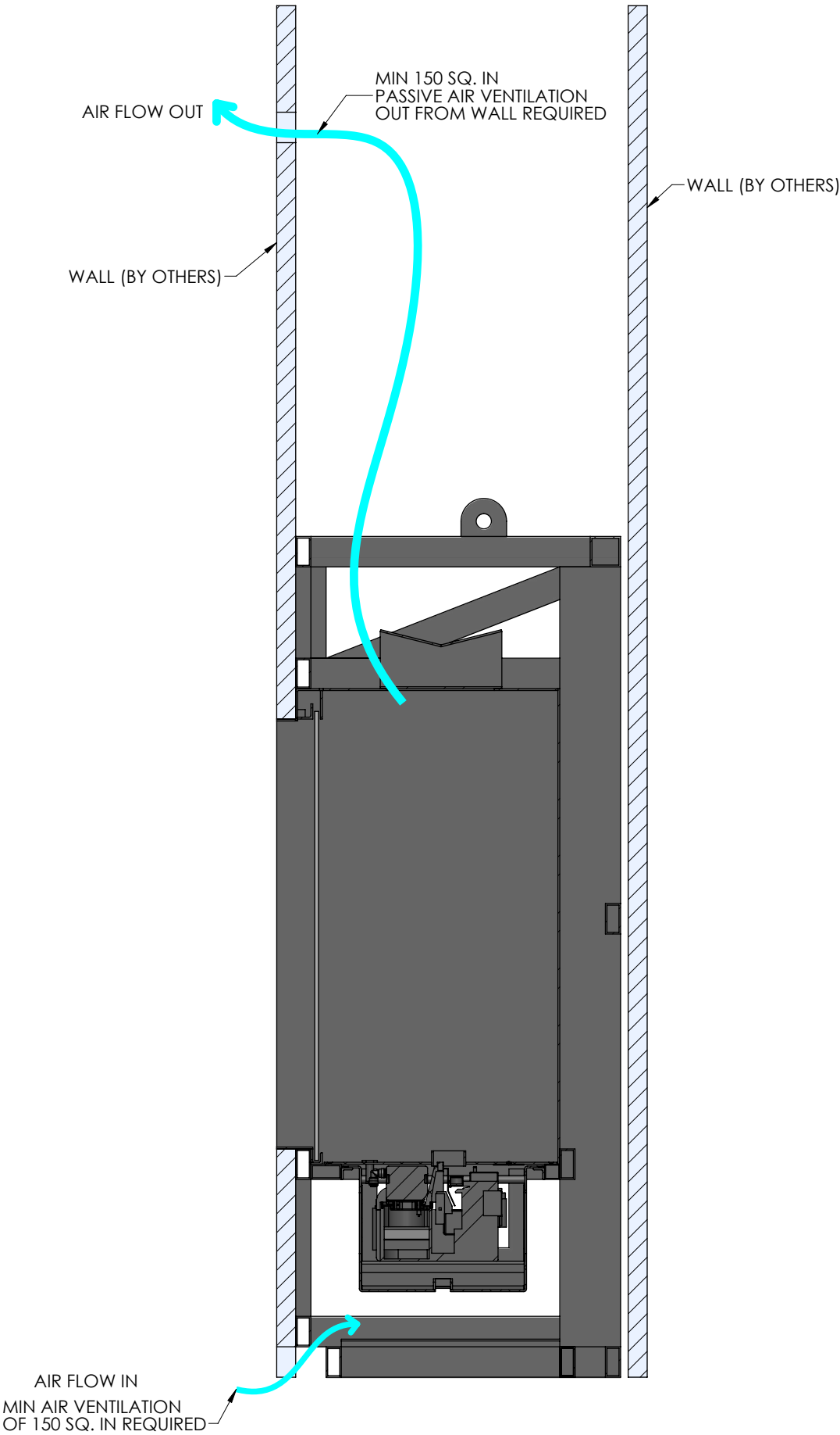
SIDE VIEW SECTION
