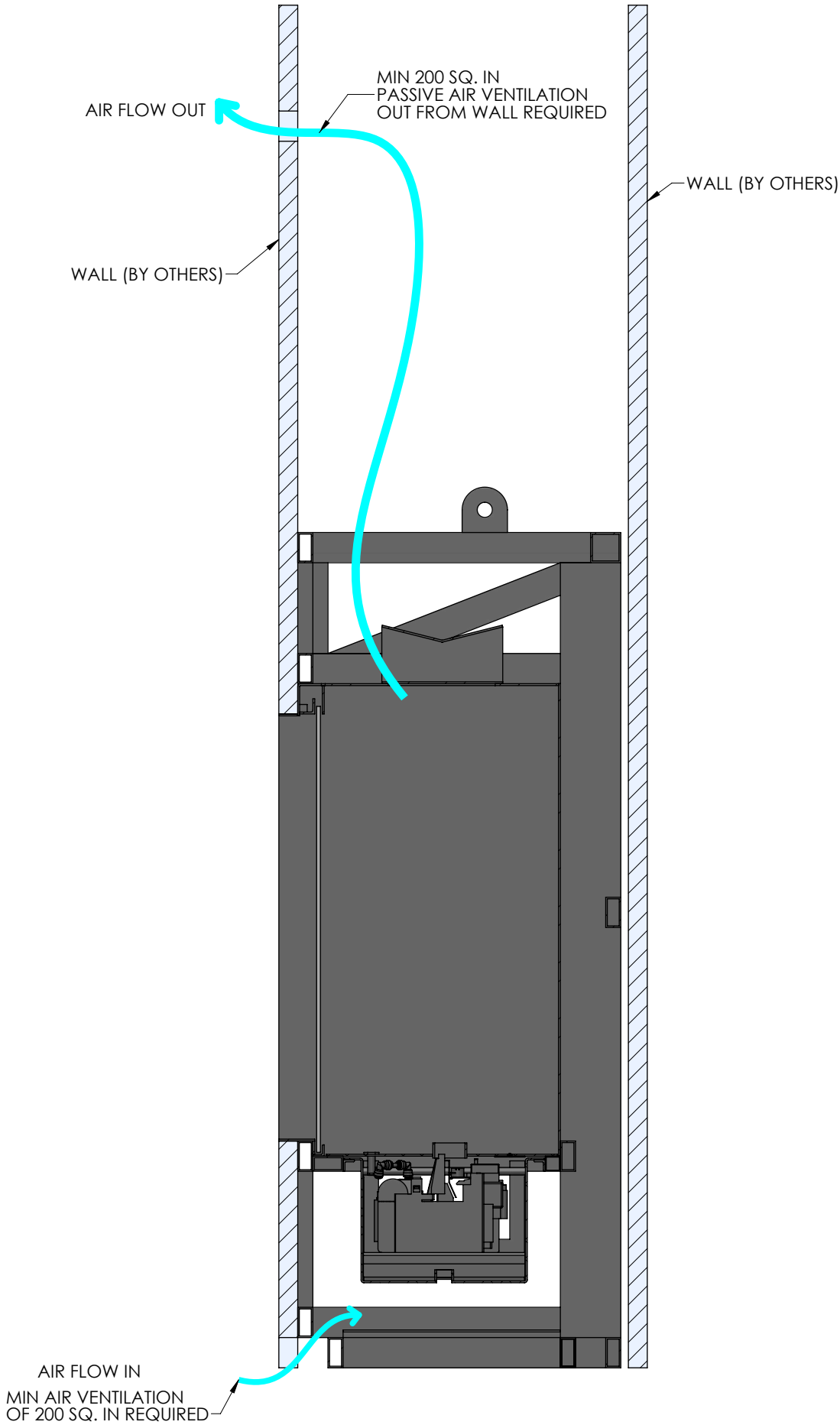
SIDE VIEW SECTION
