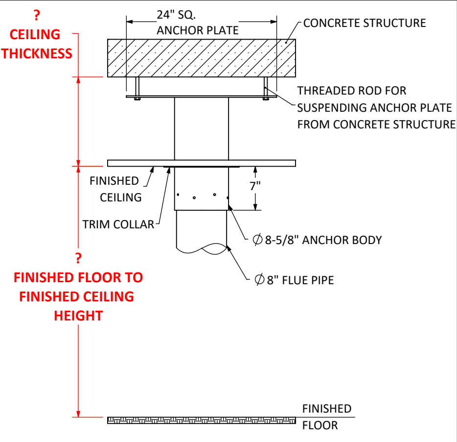
OPTION B - SUSPENDED FROM CONCRETE
